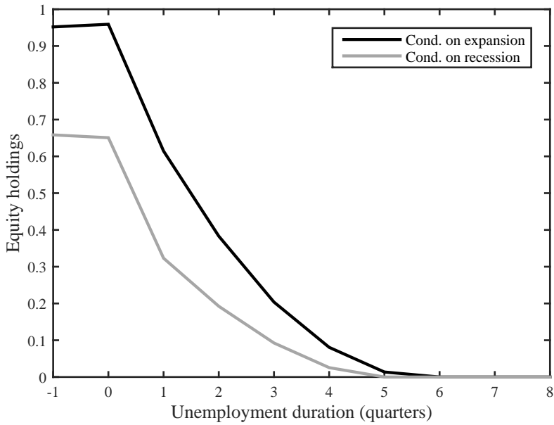
Figure 13: Post displacement equity holdings.
